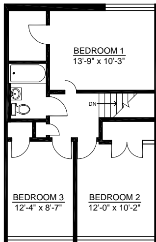
SECOND FLOOR 612 SQ.FT.
