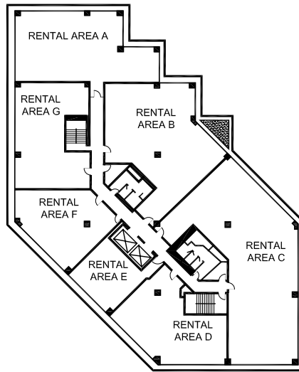
TYPICAL MULTI-TENANT FLOOR PLAN
